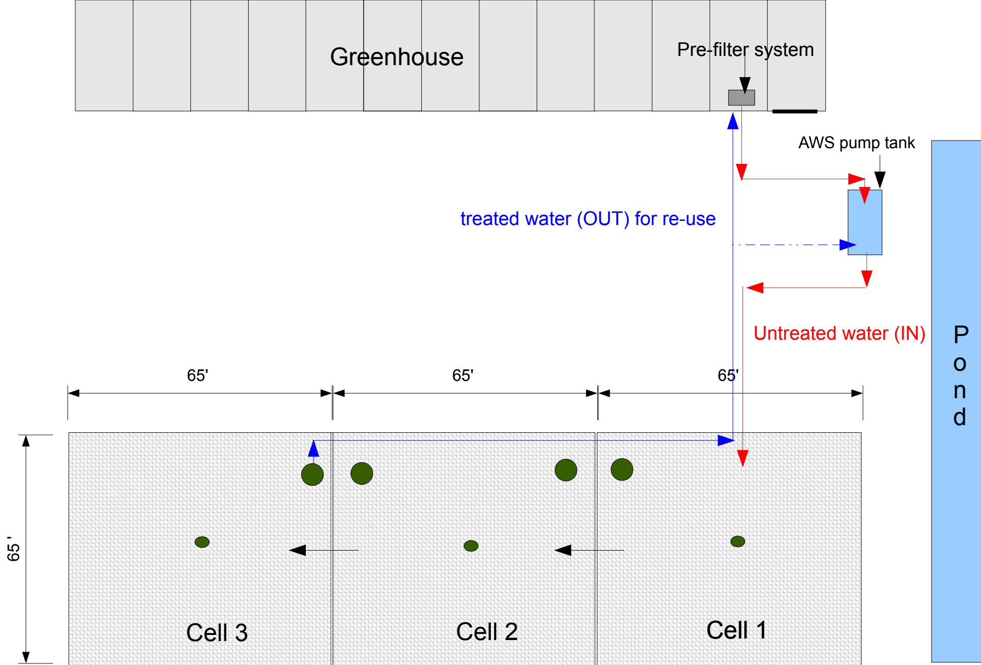
AQUA Wetland System (AWS)
